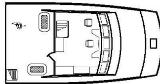
PILOT HOUSE PLAN
