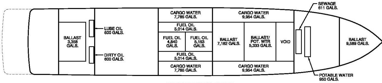
TANK ARRANGEMENT
