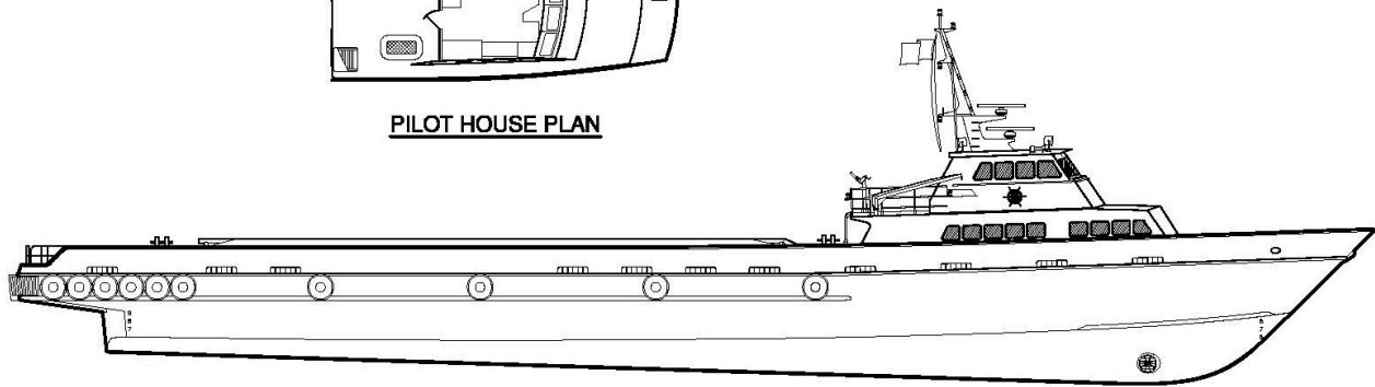
OUTBOARD PROFILE
