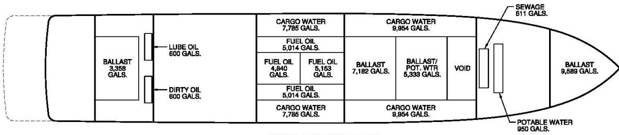
TANK ARRANGEMENT
