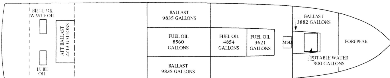
TANK ARRANGEMENT PLAN
