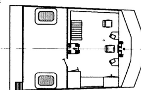
UPPER DECK AND PILOTHOUSE
