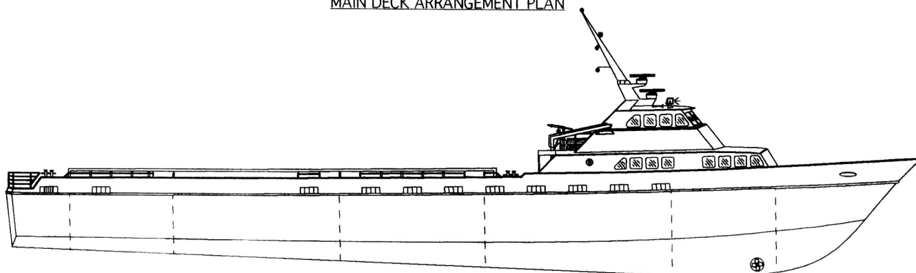
OUTBOARD PROFILE
