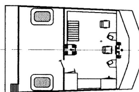
UPPER DECK AND PILOTHOUSE
